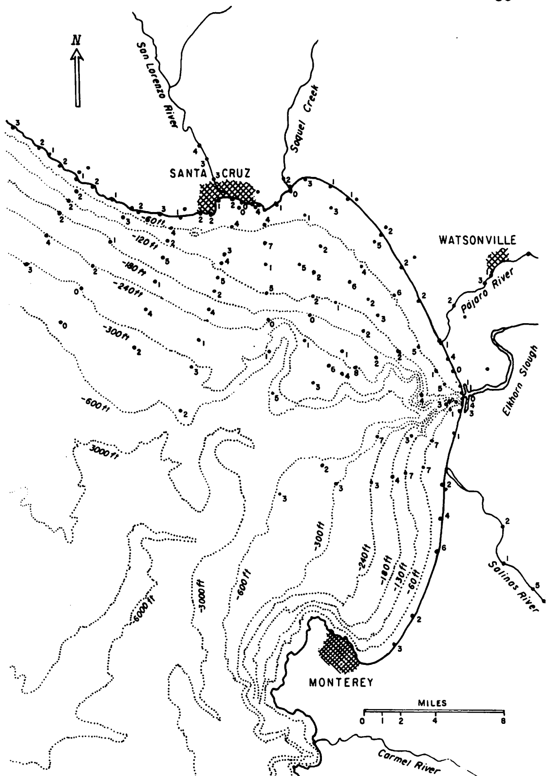
FIG. 26 CHART OF SPHERE PERCENTAGES
