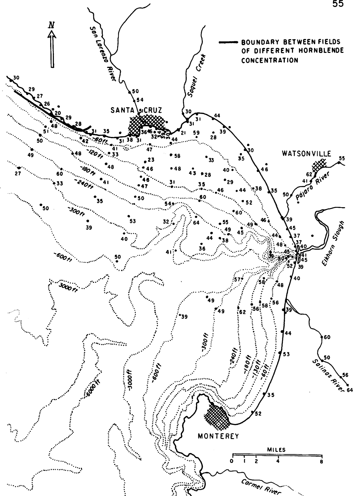
FIG. 15 CHART OF GREEN HORNBLENDE PERCENTAGES
