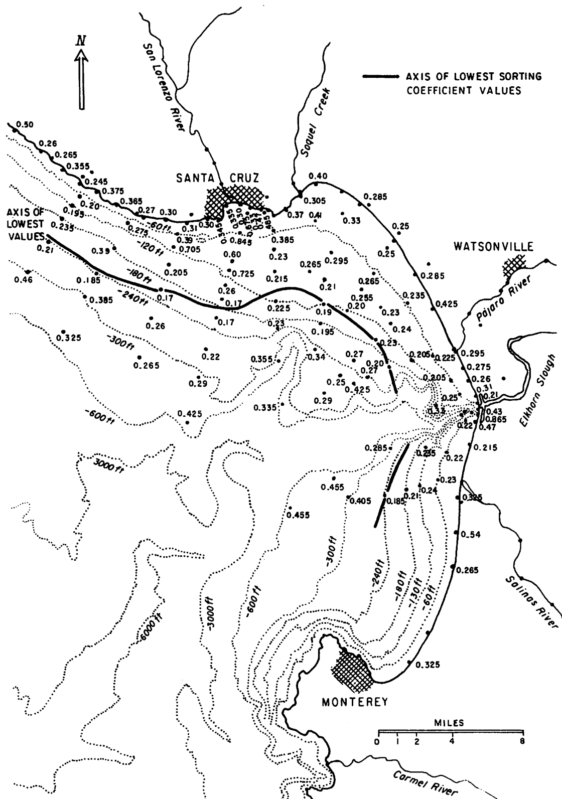
FIG. 8 PHI SORTING COEFFICIENT \left[ S_0 = \frac{Q_3\phi - Q_1\phi}{2} \right] OF SAND FRACTION OF BEACH AND MARINE SAMPLES
