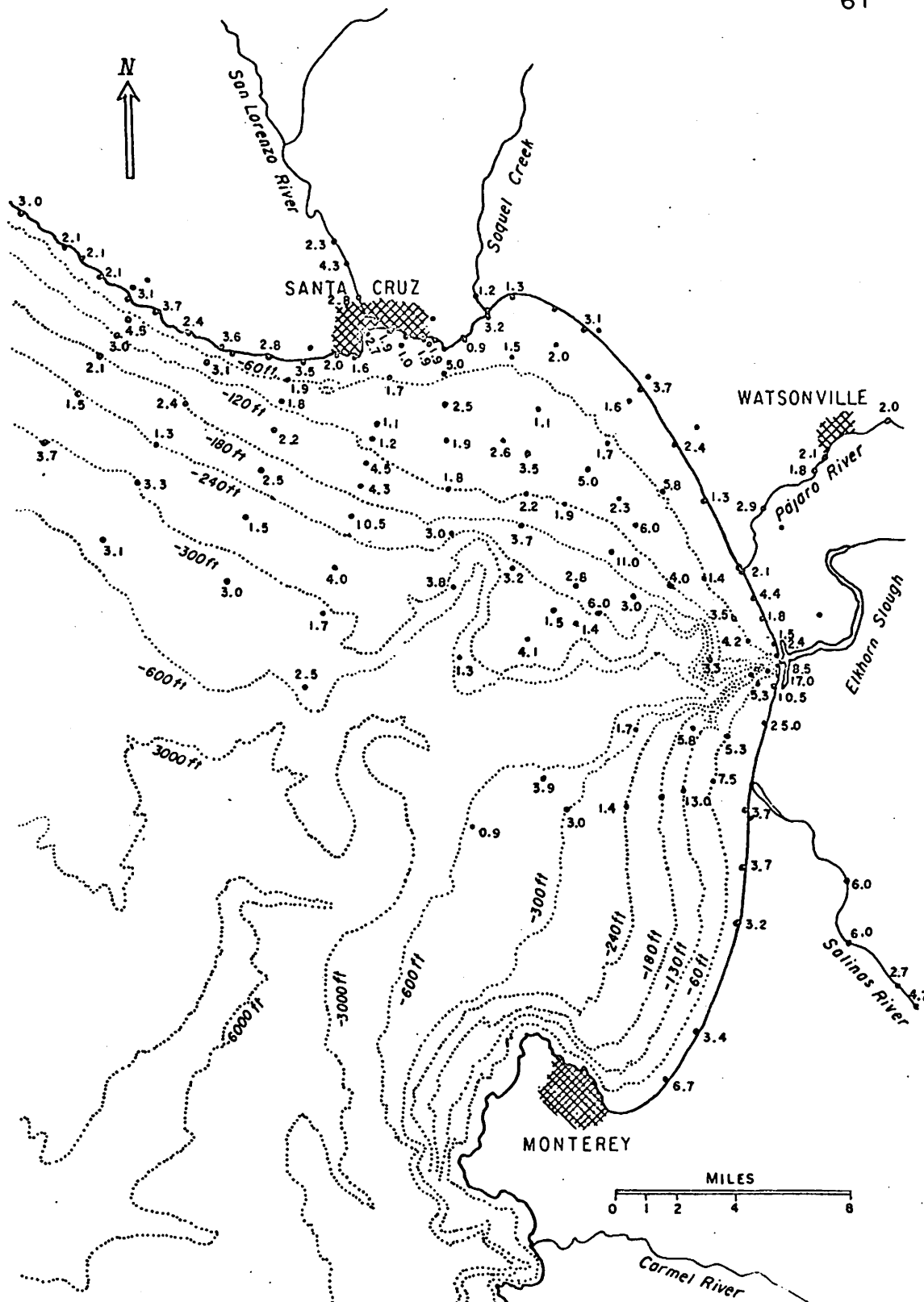
FIG. 21 CHART OF THE AUGITE/HYPERSTHENE RATIO VALUES
