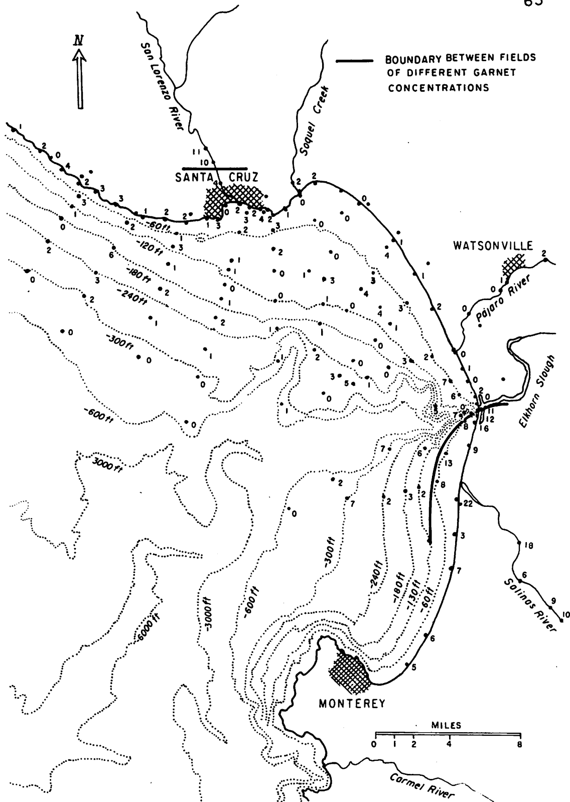
FIG. 23 CHART OF GARNET PERCENTAGES
