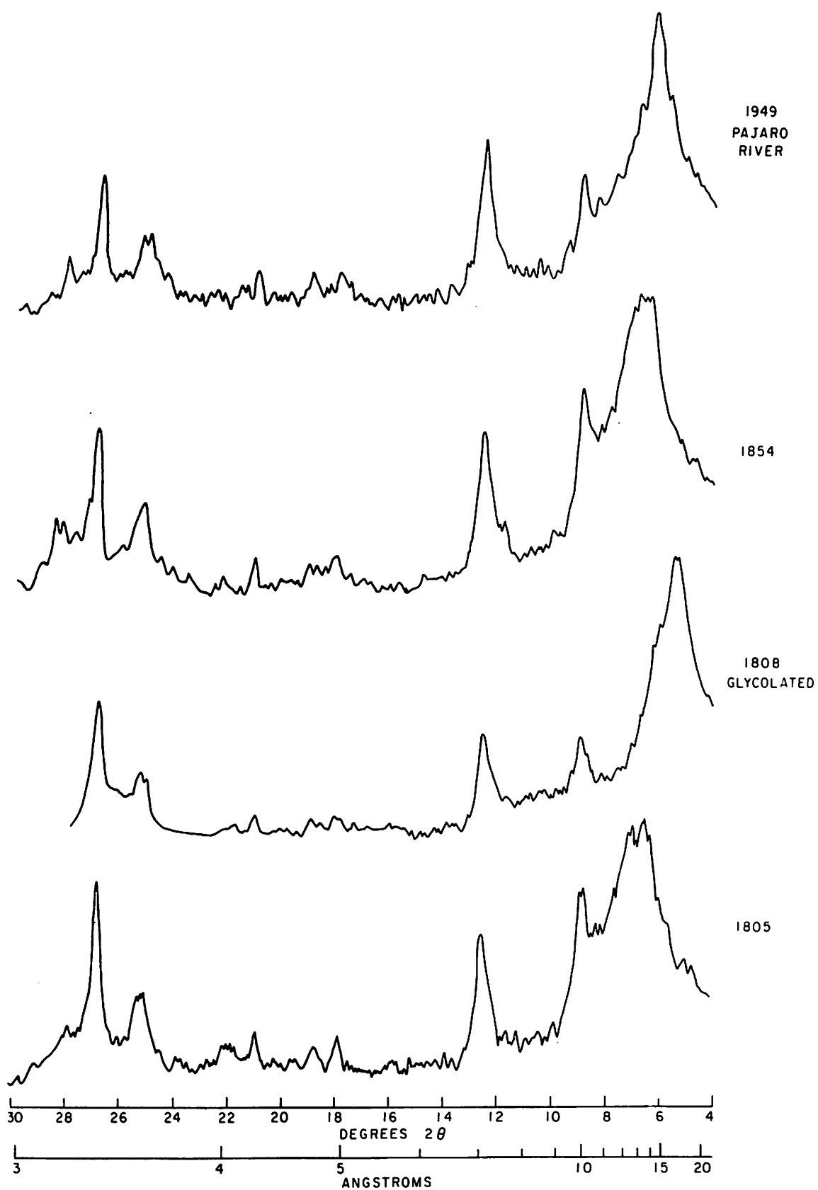
FIG 12 X-RAY DIFFRACTION DIAGRAMS (Cu Kα) OF MONTEREY BAY CLAYS
